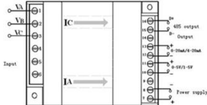
Figure 3, CE-AJ31-3**DS5 3-phase 3-wire wiring diagram
