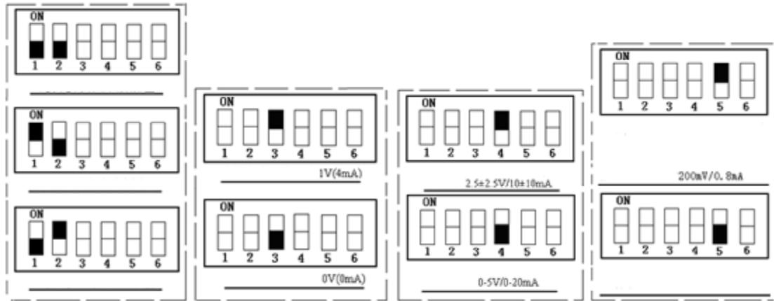
Figure 4 Measurement function settings; Figure 5 Zero output settings; Figure 6 Polarity measurement settings; Figure 7 Non-polar bias measurement
