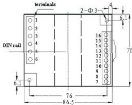
Figure 2, Guide rail mounting dimensions
