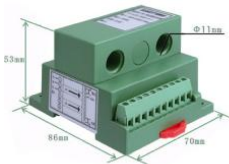
Figure 1, CE-AJ31-3**DS5 type product shape
