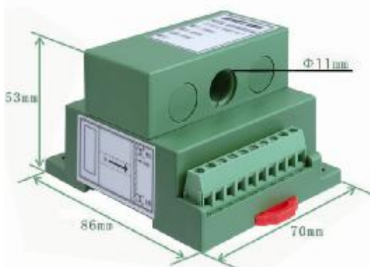
Figure 5.5 CE-AJ1*-*DS5 type product shape
