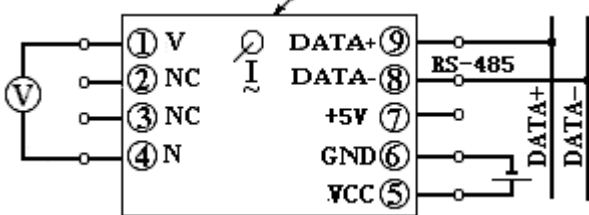
Figure 6.1 Single-phase CE-AJ11-**BS3 wiring diagram
