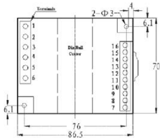
Figure 5.4 CE-AJ1*-*MN1 product installation diagram
