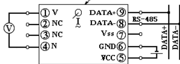
Figure 6.2 Single-phase CE-AJ12-**BS3 wiring diagram
