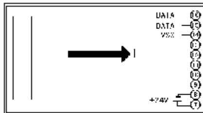
Figure 6.3 Single-phase CE-AJ12-**MN1 Product Wiring Reference Drawing
