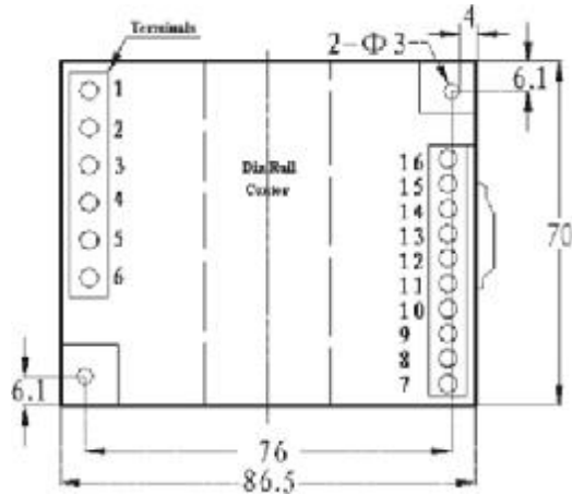
Figure 5.8 CE-AJ1*-**ES5 product installation diagram
