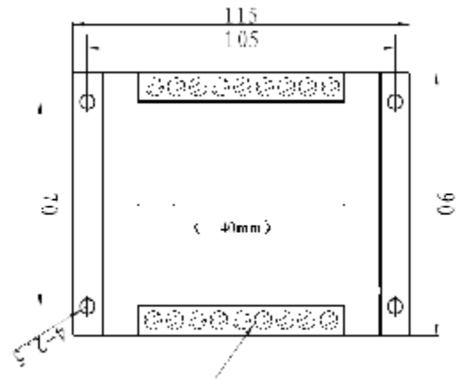
Figure 5.4 CE-AJ1*-*MN1 product installation diagram
